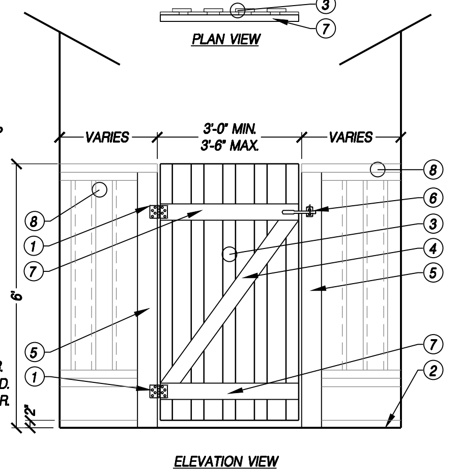
B WOOD GATE (BOARD-ON-BOARD) NTS P-SW-02
